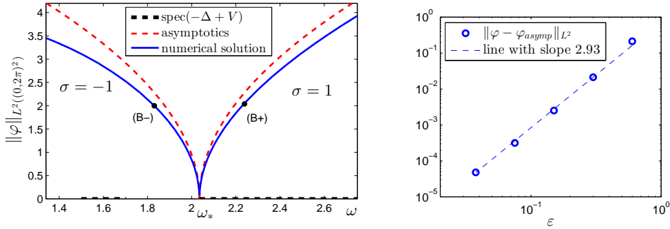
FIGURE 5. Left: Bifurcation diagram in the (\omega, \|\varphi\|_{L^2(\mathbb{P}^2)}) -plane for example B: N = 2 , k_*^{(1)} = (1/2, 0) , k_*^{(2)} = (0, 1/2) . Full lines: numerically computed solution \varphi ; dashed lines: asymptotic approximation \|\varphi\|_{L^2(\mathbb{P}^2)} \sim \sqrt{(\omega - \omega_*)/\Omega} \|\sum_{j=1}^2 A_j \xi_2(\cdot, k_*^{(j)})\|_{L^2(\mathbb{P}^2)} with \Omega = \sigma = \pm 1 . Right: error for \sigma = -1 , \varphi_{asympt} := \varepsilon \sum_{j=1}^2 A_j \xi_2(x, k_*^{(j)}) .
