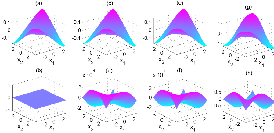
FIGURE 4. Nonlinear Bloch waves for example A. (a) and (b): real and imaginary part of the approximation \varepsilon A \xi_1(x, (1/2, 1/2)) at \varepsilon = 0.12 ; (c) and (d): real and imag. part of \varphi at (A1-) in Fig. 3; (e) and (f): real and imag. part of \varphi at (A1+) ( \sigma = 1 and \omega = \omega_* + \sigma\varepsilon^2 ); (g) and (h): real and imag. part of \varphi at (A2+)
