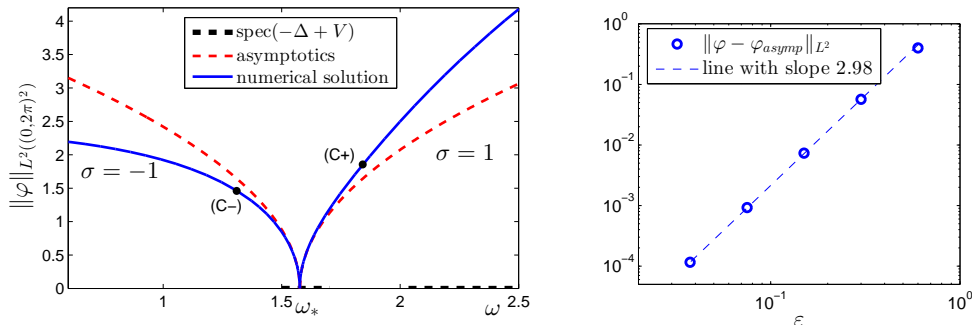
FIGURE 7. Bifurcation diagram in the (\omega, \|\varphi\|_{L^2(\mathbb{T}^2)}) -plane and error for \sigma = -1 for example C: N = 2, k_*^{(1)} = (1/4, 1/4), k_*^{(2)} = -k_*^{(1)} .
