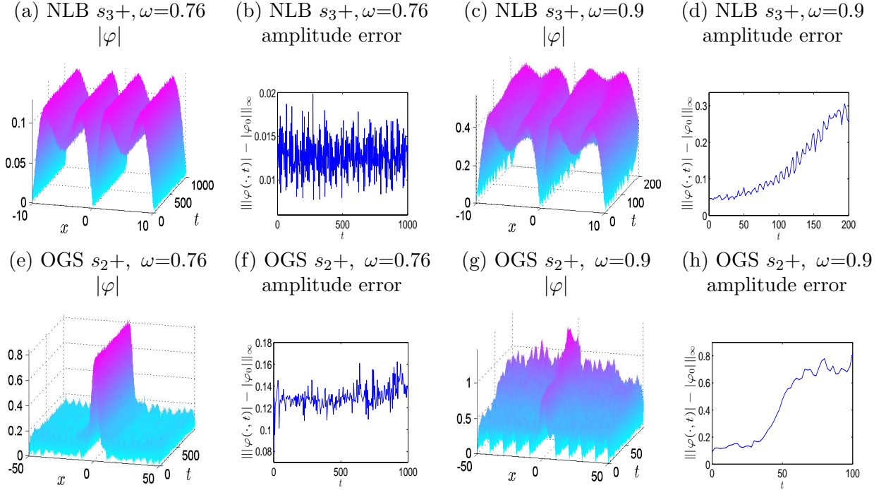
FIGURE 12. Numerical integration of (8.2) with initial data as random 10% perturbations of the indicated NLB in (a)-(d) and OGS in (e)-(h). The NLB-branch s_3+ appears stable at bifurcation and unstable otherwise. The OGS family s_2+ entering the spectrum at \omega = s_3 seems to inherit the (in)stability of the NLB.
