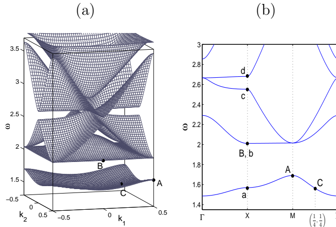
FIGURE 1. (a): Band structure of L over the Brillouin zone \mathbb{B} for the periodic potential (1.4); (b): along the boundary \Gamma - X - M - \Gamma of the, so called, irreducible Brillouin zone.
