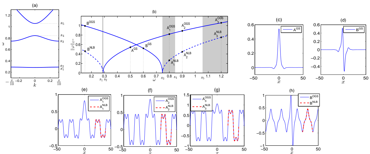
FIGURE 9. Panel (a): the band-structure for V(x) = \sin^2(\frac{\pi x}{10}) ; (b): a bifurcation diagram of GS and NLBs for (1.2) in 1D, \sigma = 1 . (c) and (d): plots of the GS at A^{\text{GS}} and B^{\text{GS}} resp.; (e)-(h): OGS and NLB at the remaining marked points.
