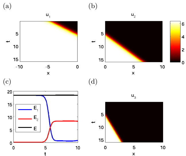
FIG. 2. (Color online). Numerical solution of (1), (2), (6), with \beta_k = 1 , k = 1, 2, 3 , and a_1 = 1 , a_2 = 0.7 , a_3 = 0.3 fulfilling (10). The initial conditions belongs to the kink (18) on bond 1 with x_0 = -5 and \nu = 0.9 , while u_{2,3} = \partial_t u_{2,3} \equiv 0 . Panels (a),(b),(d) arranged corresponding to Fig. 1, while (c) shows the t -dependence of the energies.
